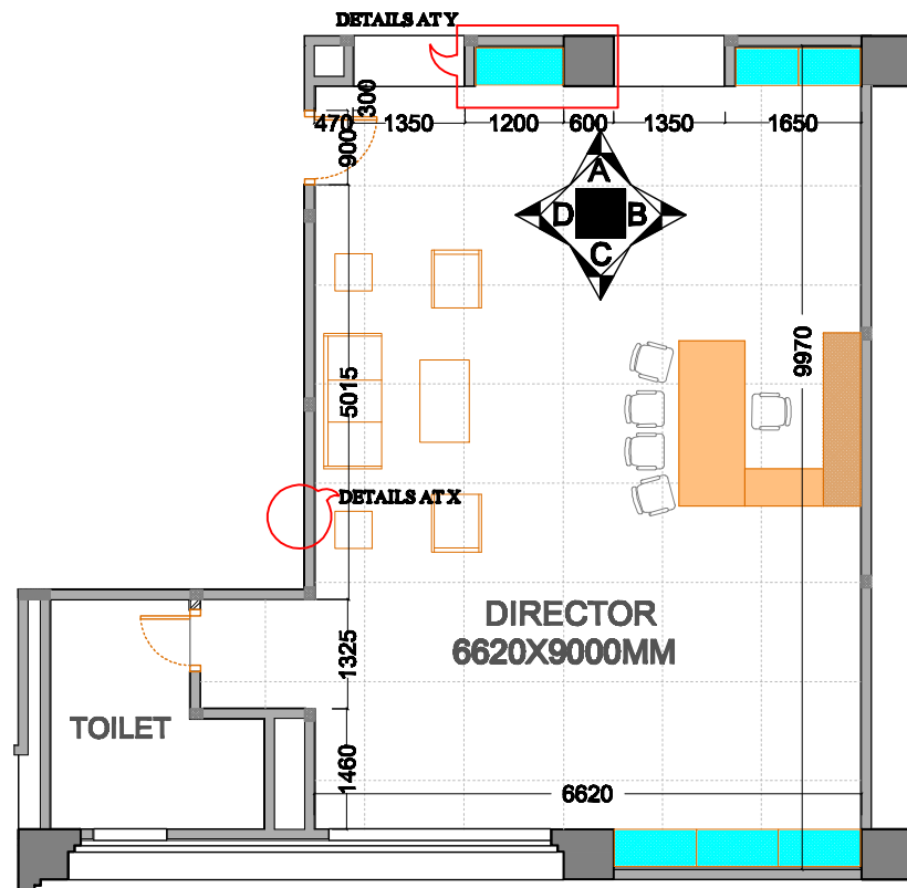
FURNITURE LAYOUT OF THE DIRECTOR'S CABIN- 1
